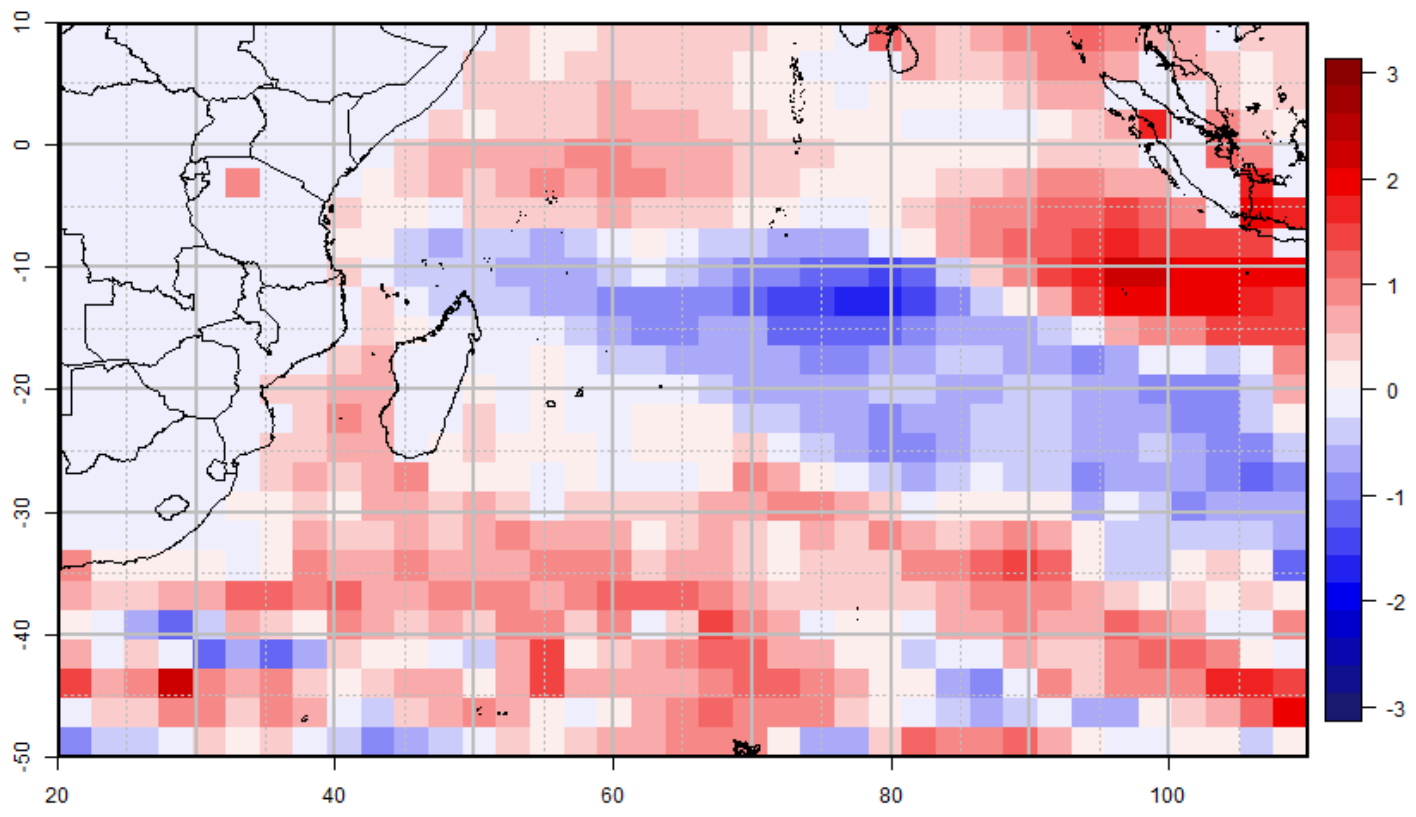
Forecast ARP SST OND 2016
