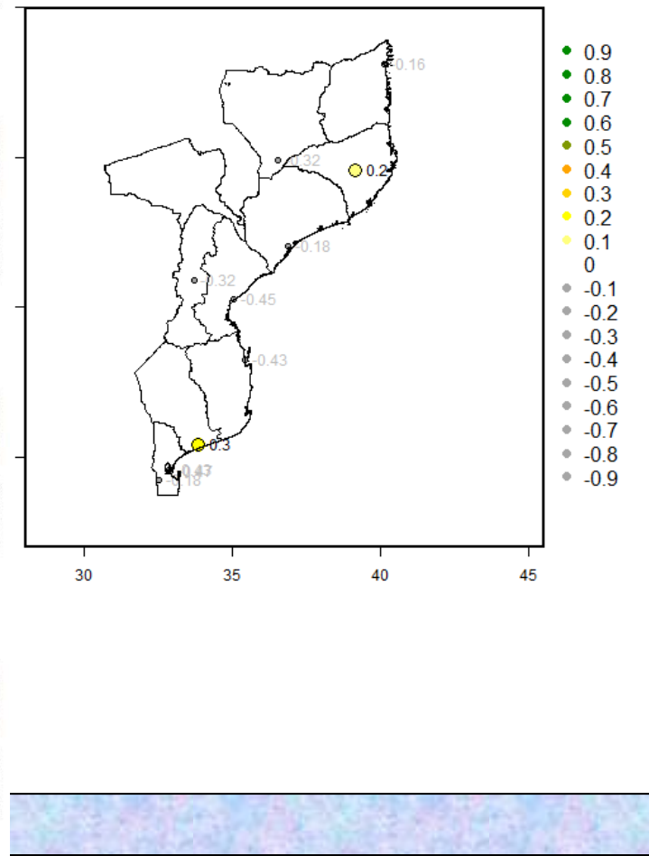
Correlation RR : obs / model ( SST OND )
