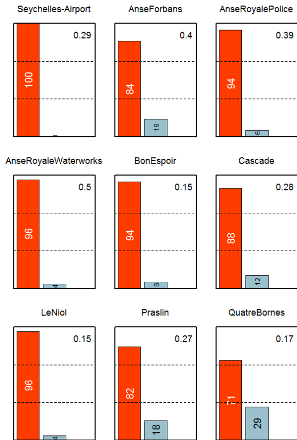
SEASONAL FORECAST : Lower tercile RR OND 2016
