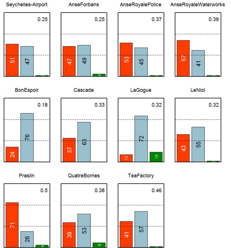
SEASONAL FORECAST: Upper tercile RR OND 2016
