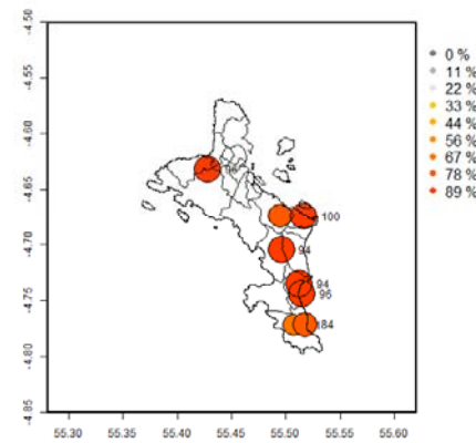
SEASONAL FORECAST : Lower tercile RR OND 2016
