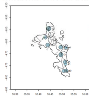
SEASONAL FORECAST: Median tercile RR OND 2016
