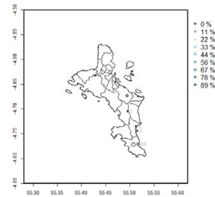
SEASONAL FORECAST : Median tercile RR OND 2016
