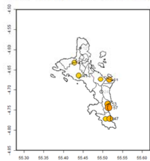
SEASONAL FORECAST: Lower tercile RR OND 2016
