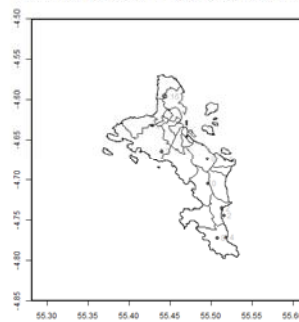
SEASONAL FORECAST: Upper tercile RR OND 2016
