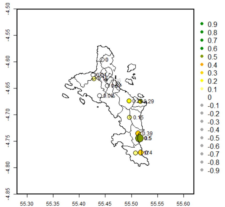
Correlation RR : obs / model ( SST OND )
