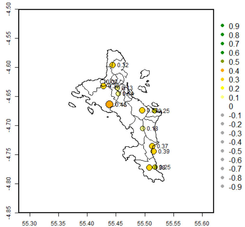
Correlation RR : obs / model ( U850 OND )
