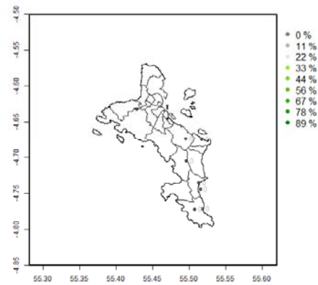
SEASONAL FORECAST : Upper tercile RR OND 2016
